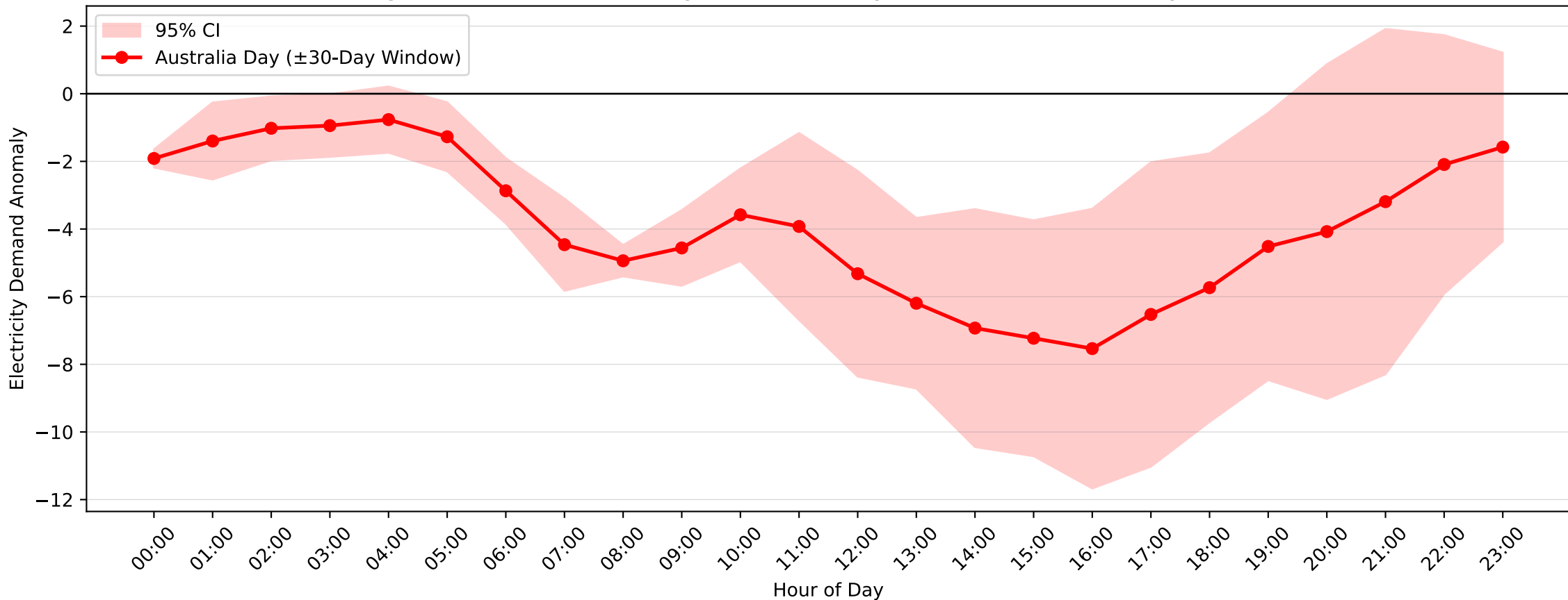
Kogarah Demand Anomaly: Australia Day (2016–2017, \pm 30 -Day Window)
