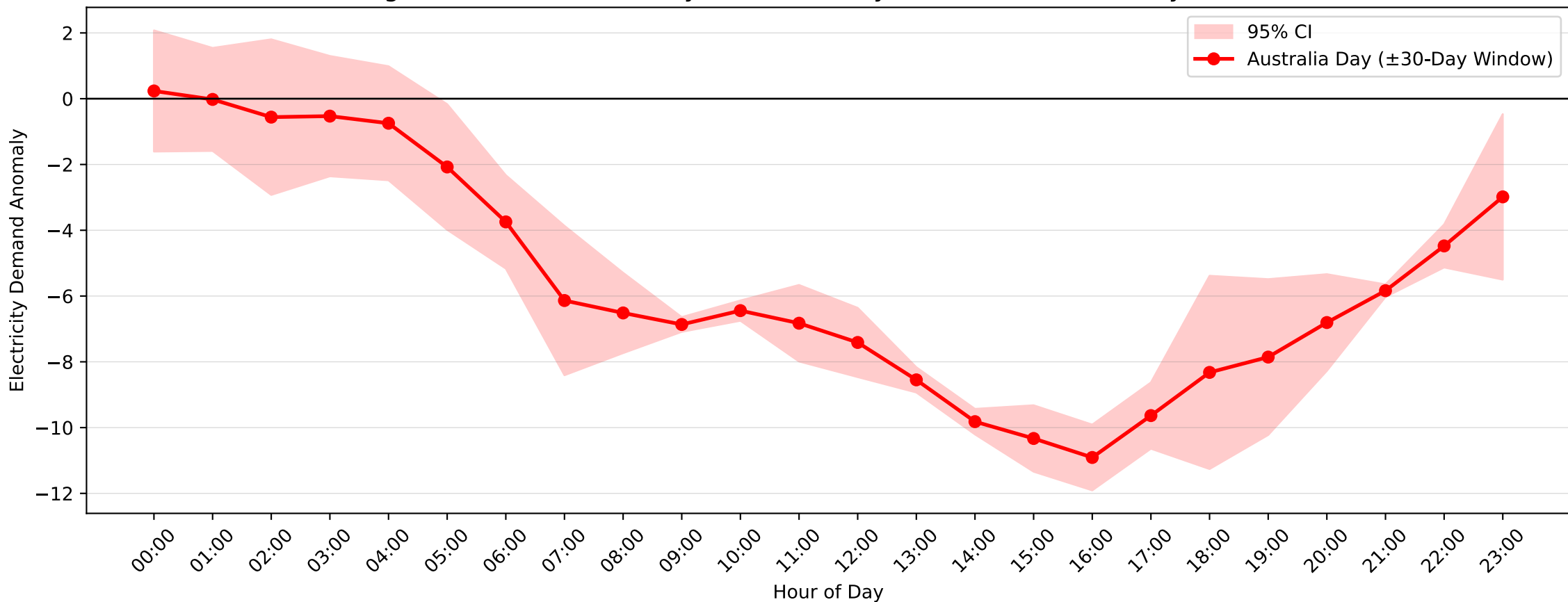
Kogarah Demand Anomaly: Australia Day (2014–2015, \pm 30 -Day Window)
